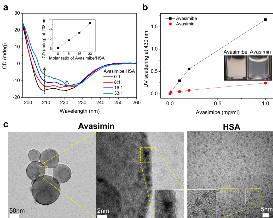
Figure 1. Water-soluble avasimibe nanomedicine, avasimin. (a) CD spectra of HSA at different avasimibe:HSA molar ratios. Inset: Plot of CD intensity at 208 nm as a function of avasimibe:HSA molar ratio. (b) Solubility measurement of avasimibe and avasimin (with 10 wt % avasimibe loading) in PBS by UV scattering at 430 nm. Inset photograph shows avasimibe (1 mg/mL) and avasimin containing the same concentration of avasimibe in PBS. (c) High-magnification TEM images of avasimin and HSA. The size, polydispersity, and zeta-potential of avasimin are 169 \pm 85 nm, 0.41, and 0.83 \pm 4.95 mV, respectively.
